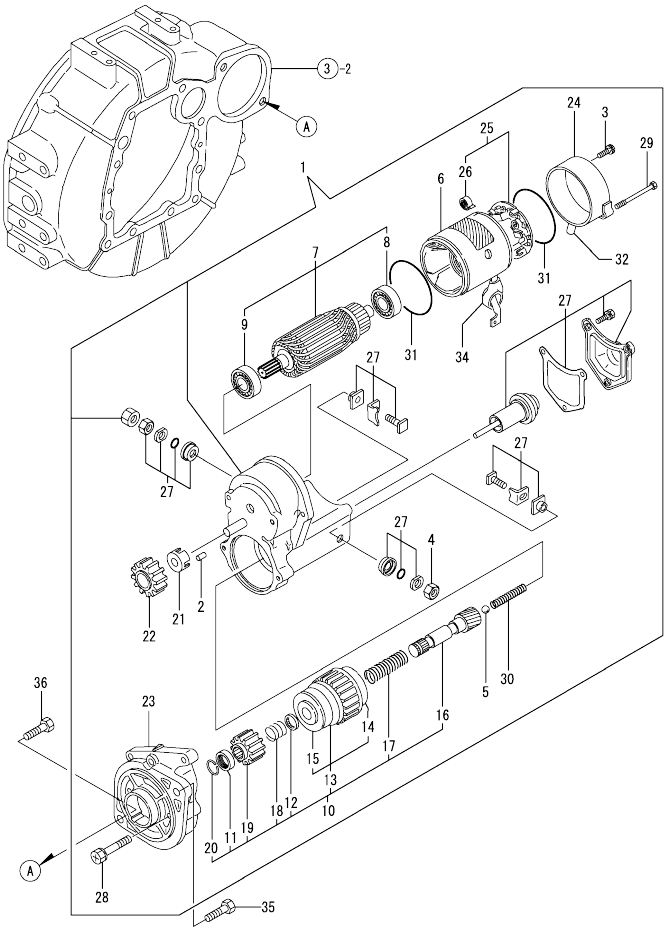
Fig.15. STARTING MOTOR
